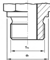
Sealing: Sealing washer DIN 7603 (e.g. copper)
