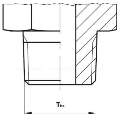
Tapered Thread
